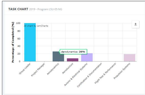
Gambar 7. Diagram Progres
