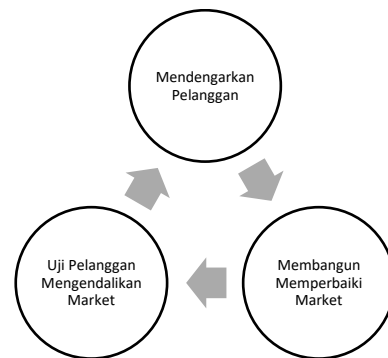
Gambar 1. Metode Prototype
