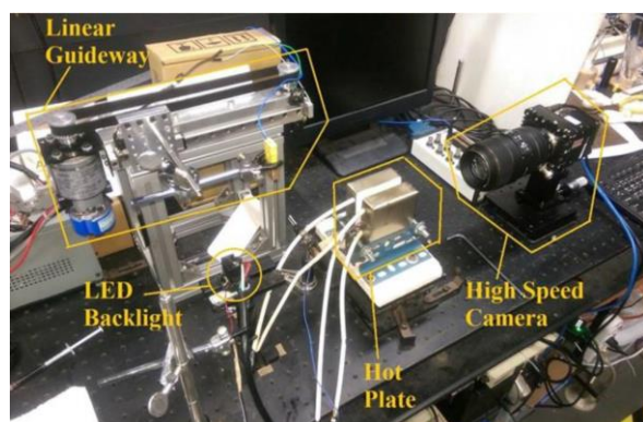
Figure 3: Suspended droplet experiment
