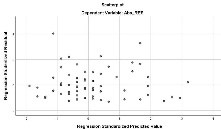
Gambar 1 Scatterplot
