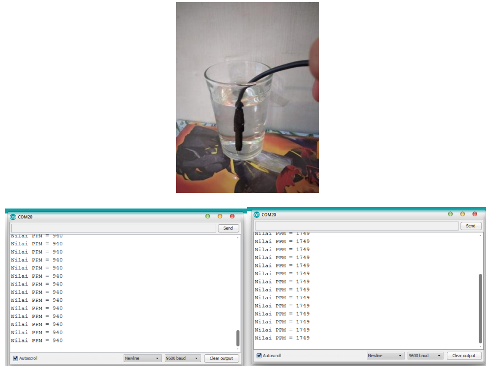
Gambar 2.6 Pengujian Sensor TDS
