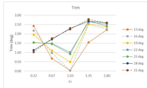
Figure 12. Trim Angle
