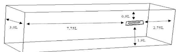
Figure 5. Fluid domain
