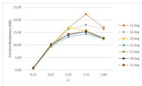
Figure 8. Friction Resistance
