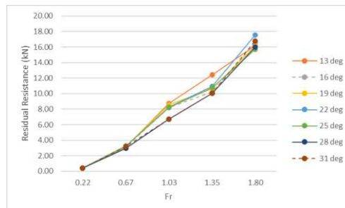
Figure 9. Residual Resistance
