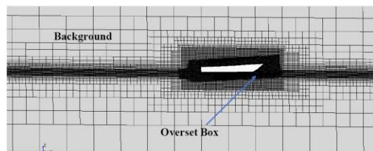
Figure 6. Overset Mesh
