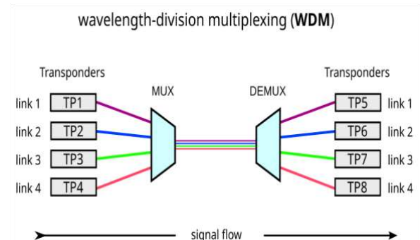
Fig.1: WDM Structure
