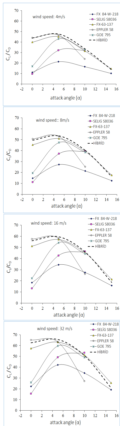
Fig. 8 Comparison of performance of hybrid airfoil with that of other airfoils at different wind speeds
