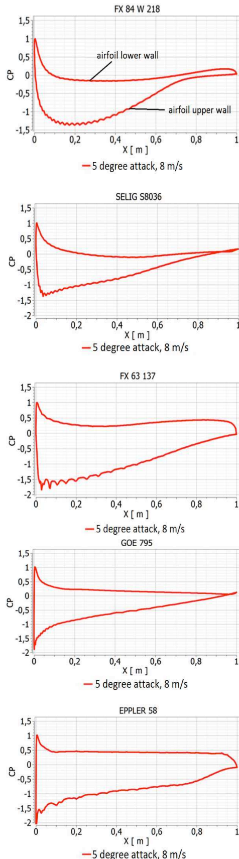
Fig. 6 Distribution of pressure on upper and bottom walls at attack angle of 5^\circ and wind speed of 8 m/s for each five airfoils
