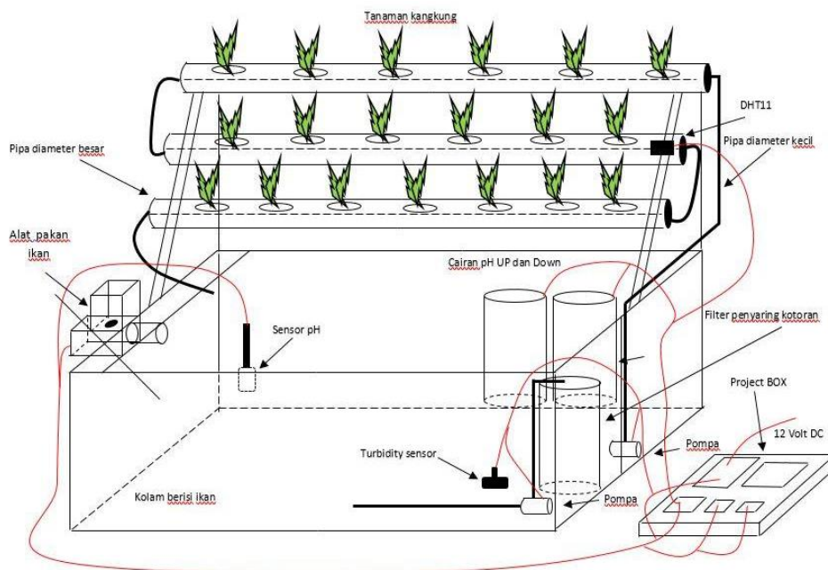
Gambar 4. Design Prototype
