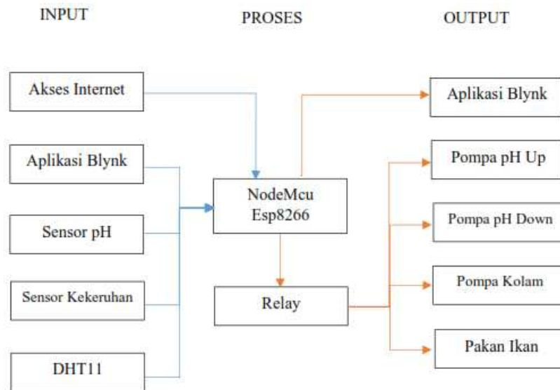
Gambar 3. Wiring Diagram System
