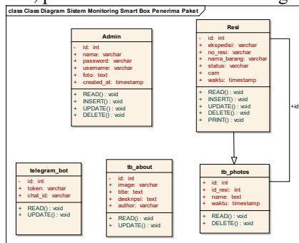
Gambar 12. Class Diagram
