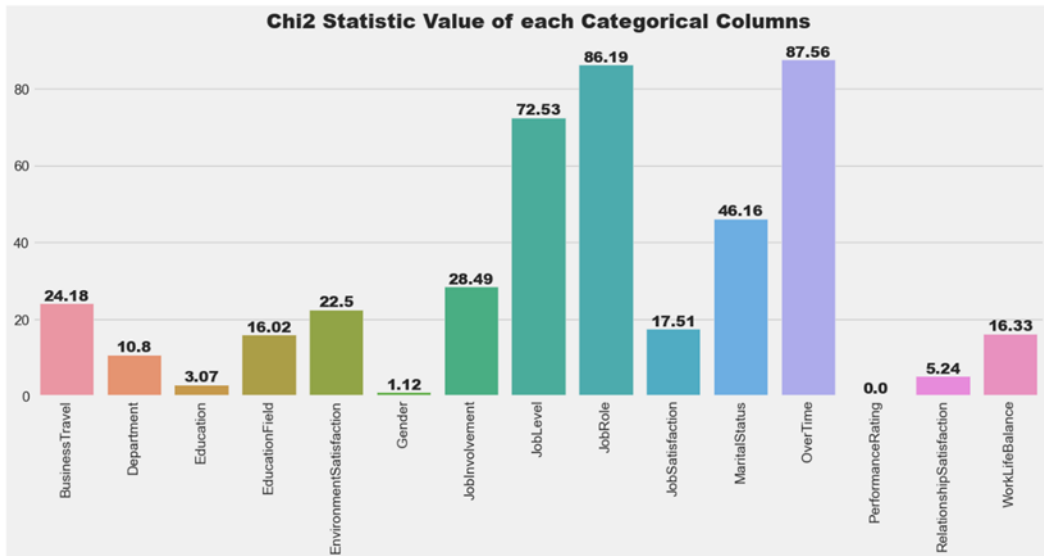
Gambar 8. Uji chi-square
