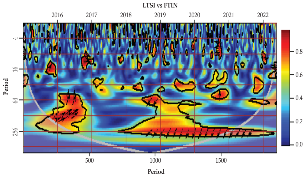
Figure 3. Continuous Wavelet Transforms: LTSI VS FTIN
