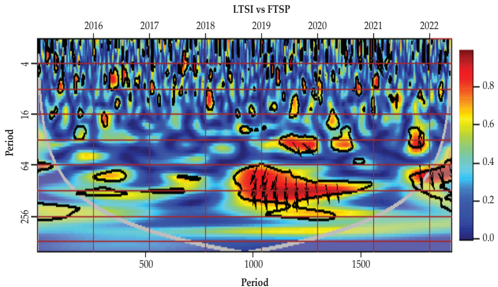
Figure 4. Continuous Wavelet Transforms: LTSI VS FTSP
