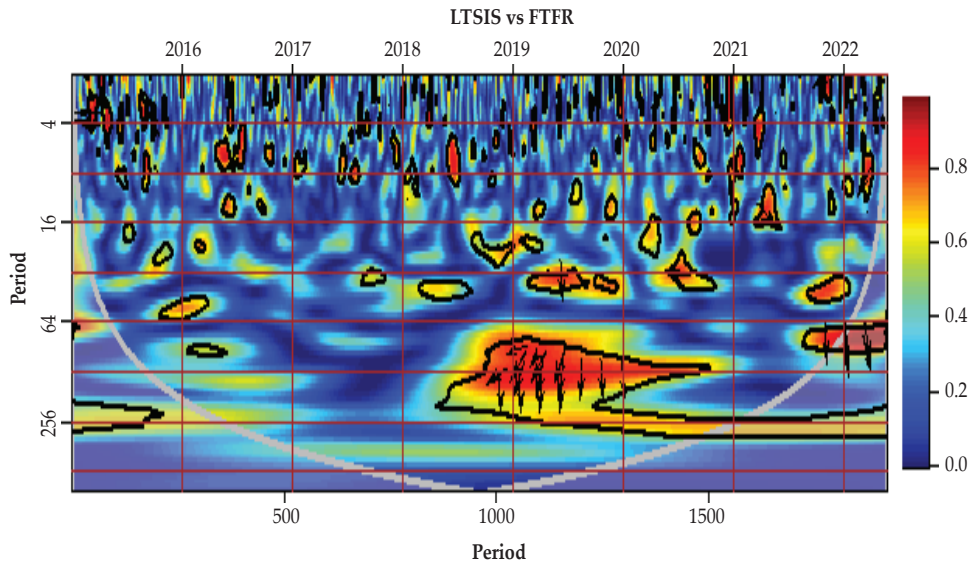
Figure 6. Continuous Wavelet Transform: LTSIS VS FTFR
