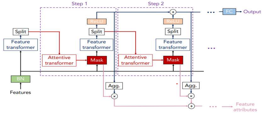
Figure 2. TabNet Architecture[6]
