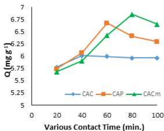
Figure 4. Effect of contact time on MB removal process.
