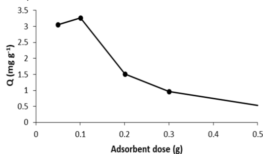
Figure 1. Effect of adsorbent dose on MB removal.
