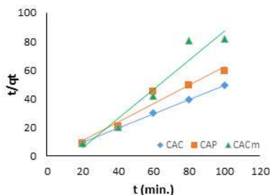
Figure 6. Pseudo-second order kinetic model parameters for adsorption of MB onto CACm, CAP, and CAC.
