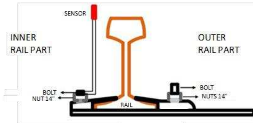
Figure 5. Device placement
