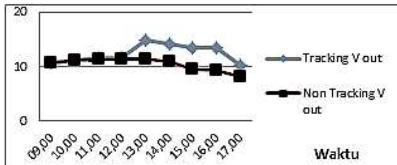
Figure 13. Graph of Voltage Difference Between V_{out} Tracking and Non Tracking
