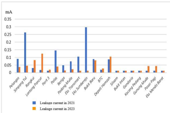
Figure 1. Leakage current
