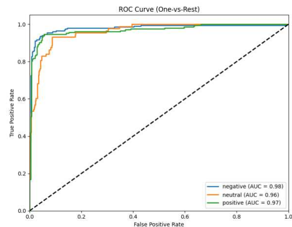
Figure 4. ROC Curve on QBC Rating-Pseudo Model
