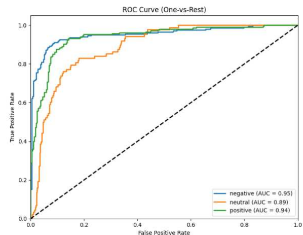
Figure 3. ROC Curve on Vader Based Model
