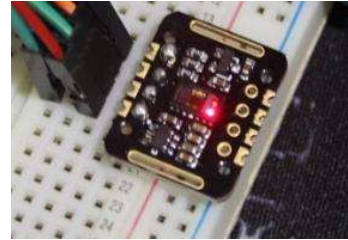
Gambar 3. MAX30102 Sensor
