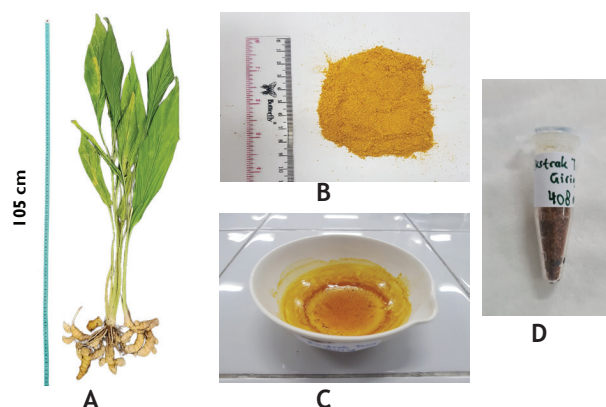
Figure 1. Extraction of C. heyneana rhizome.
