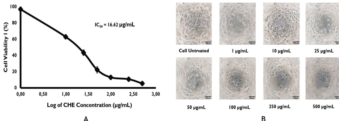
Figure 5. CHE Cytotoxicity Profile on JHH-4 cells. 2.500 of JHH4 cells were seeded in each well on a 96-well plate and treated with serial concentrations of CHE (1-500 µg/mL) for 24 h. Cytotoxic test was carried out using the MTT Assay method. (a) Viability profile of JHH4 cells due to CHE treatment and obtaining IC_{50} of 16.62 µg/mL; (b) JHH-4 cells morphology after being treated.
