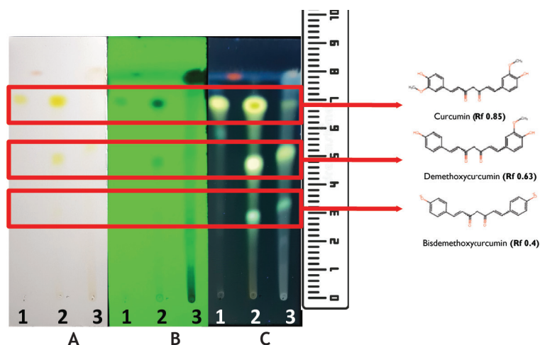
Figure 2. Chromatogram Profile. Standard curcumin 1 mg/mL, curcuminoid standard 1 mg/mL, and 15 mg/mL Curcuma heyneana extract (CHE) were eluted in a mixture of chloroform and methanol (19:1) with silica gel plate stationary phase F254 (Merck). The confirmed extract contains curcumin at Rf 0.85, demethoxycurcumin with Rf 0.63, and bisdemethoxycurcumin with Rf 0.4 as seen in the visualization of A. visible light; B. uv 254 nM, C. uv 366 nM. 1. standard curcumin 1 mg/mL; 2. standard curcuminoids 1 mg/mL, and 3. CHE 15 mg/mL.
