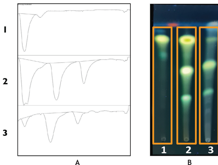
Figure 3. Intensity band curve from TLC results at 366 nM UV light. TLC results on 366 nM UV light were measured on the intensity band using the ImageJ software by measuring spot area on standard curcumin 1 mg/mL, standard curcuminoid extract 95% 1 mg/mL, and CHE 15 mg/mL. A. Intensity band curve from TLC results; B. TLC results at 366 nM UV light.
