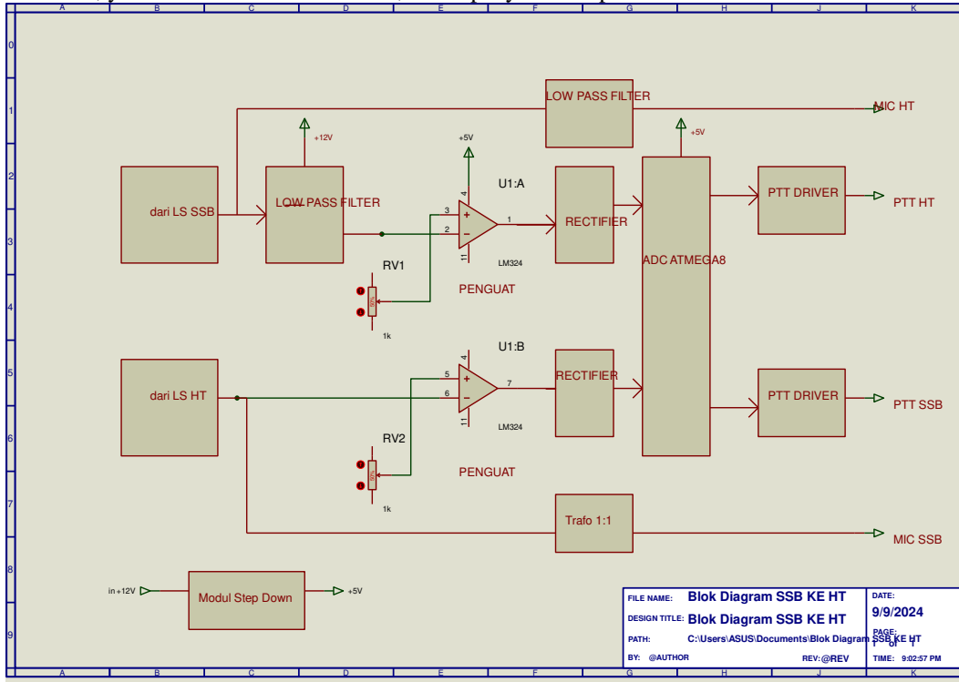
Gambar 8 Blok diagram interface
