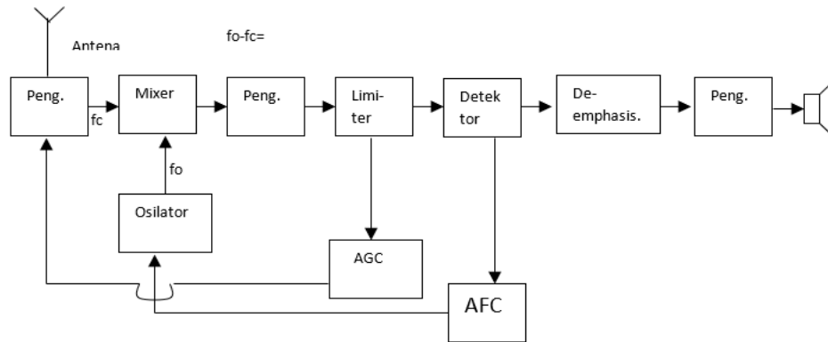
Gambar 3 Blok Diagram Penerima FM
