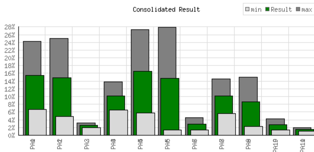
Gambar 5. Eigen Vector
