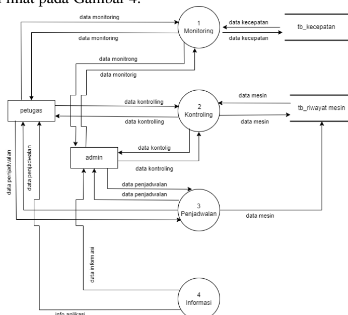
Gambar 4. Data Flow Diagram
