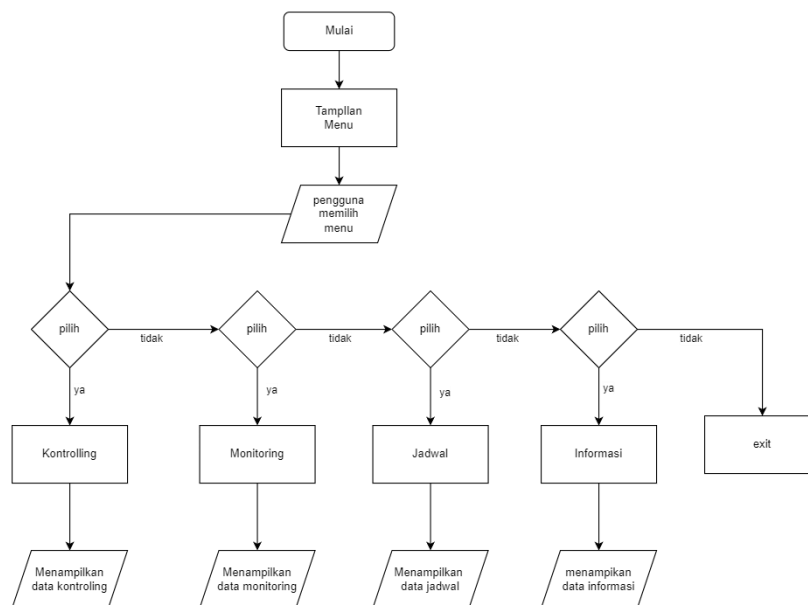
Gambar 3. Flowchart
