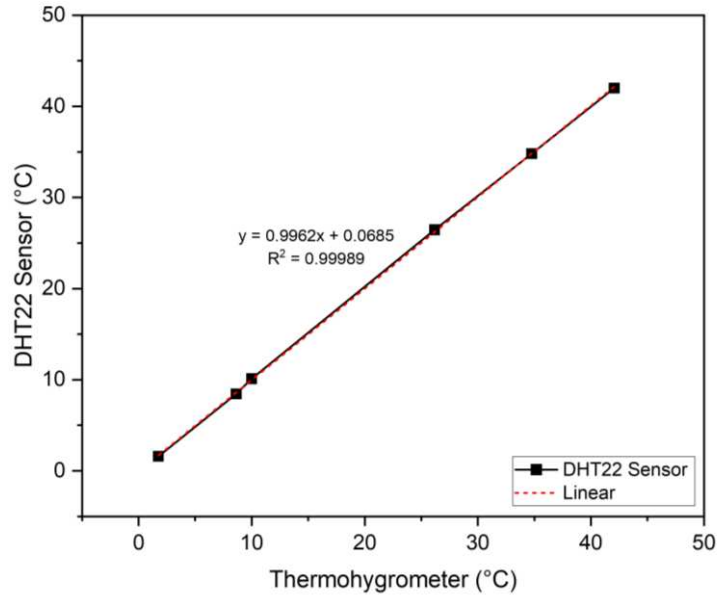
Figure 6 Calibration results of the DHT22 temperature sensor.
