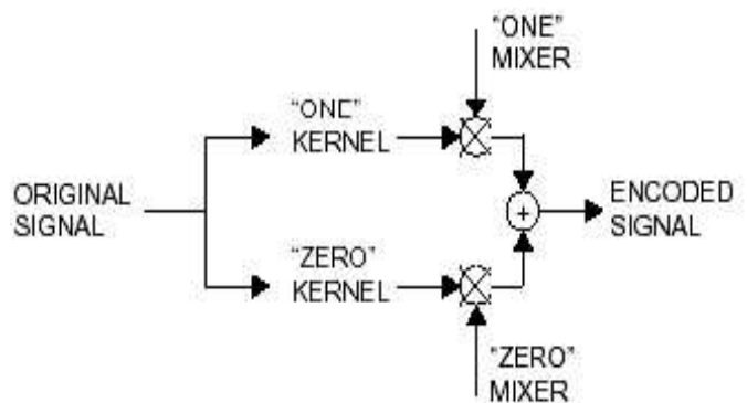
Gambar 5. Proses encoding
