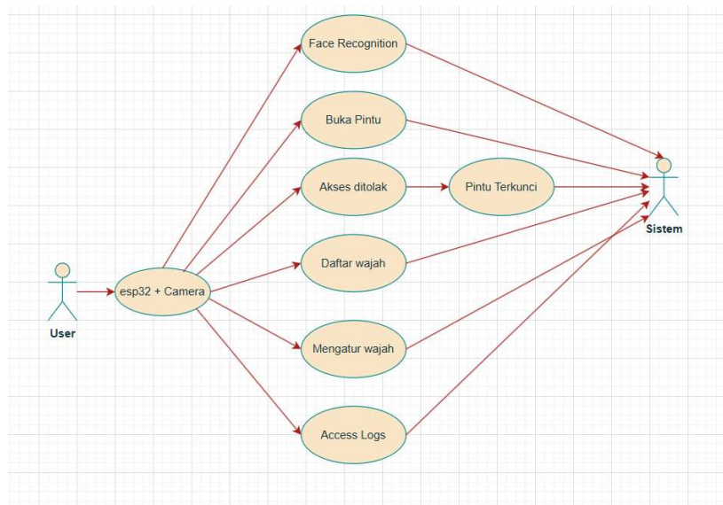
Gambar 2. Use Case Diagram Sistem Pengamanan Smarthome
