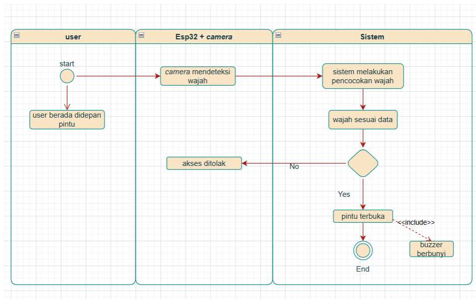
Gambar 3. Activity Diagram Sistem Pengamanan Smarthome
