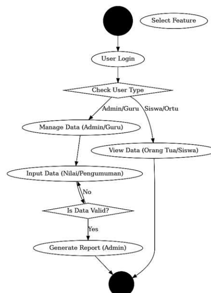
Gambar 5. Flowchart
