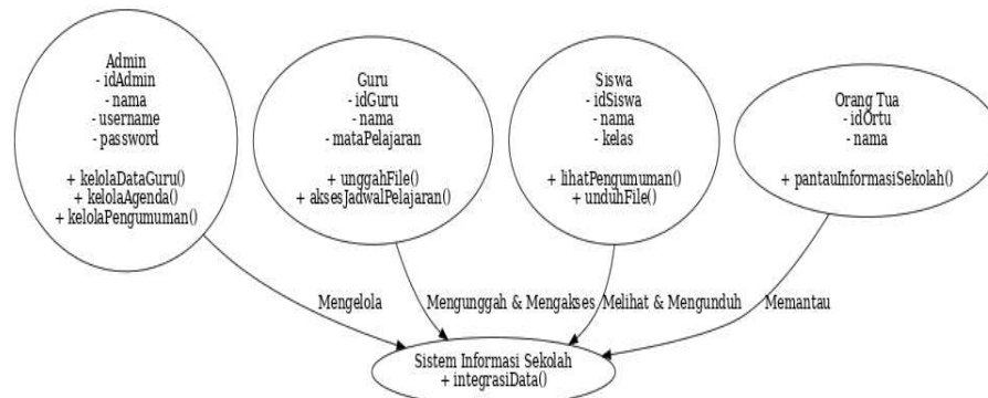
Gambar 4. Diagram Class
