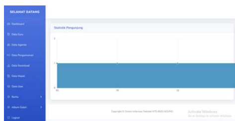
Gambar 13. Tampilan Dashboard
