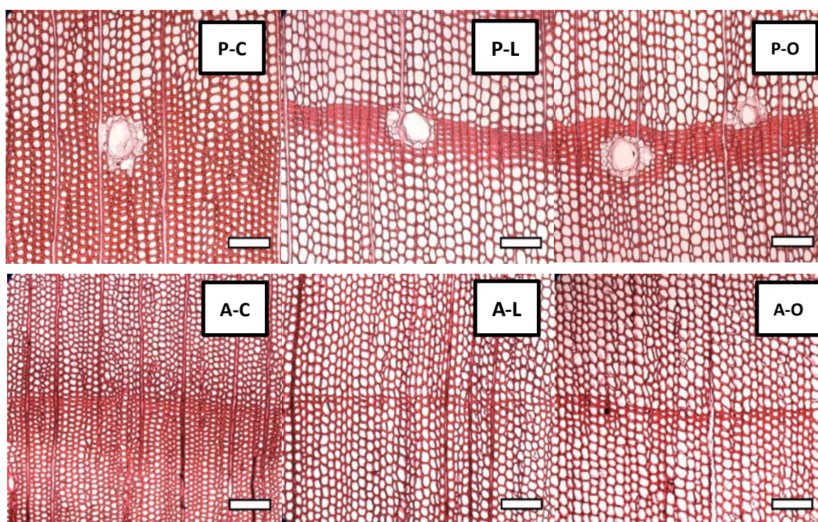
Fig. 2. Optical micrographs of the cross-section in CW, LW, and OW of Sumatran pine (P-C, P-L, and P-O) and Agathis (A-C, A-L, and A-O), respectively. – Scale bars= 200 µm.
