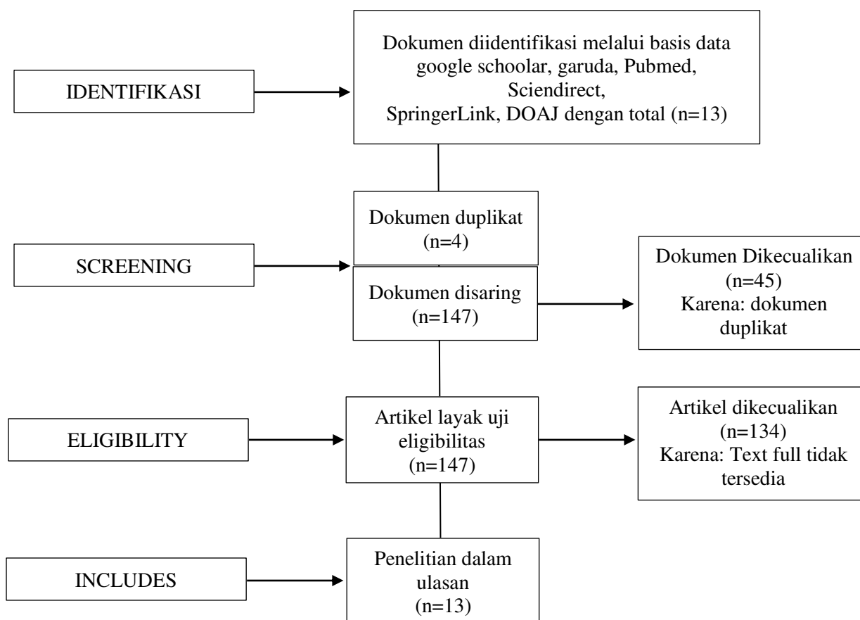
Gambar 1. Prisma Flowchart
