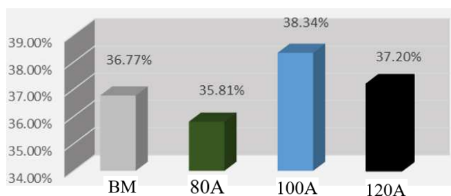
Fig. 10. Elongation diagram
