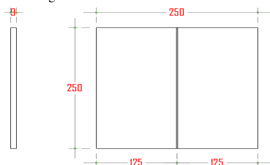
Fig. 2. Material Dimensions
