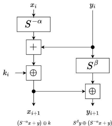
Gambar 1. Round Function Algoritma Speck. Sumber: (Sleem and Couturier, 2021)
