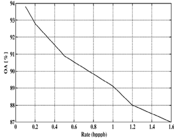
Figure 7. Classification accuracy of DWT-CP using SVM (RBF Kernel).
