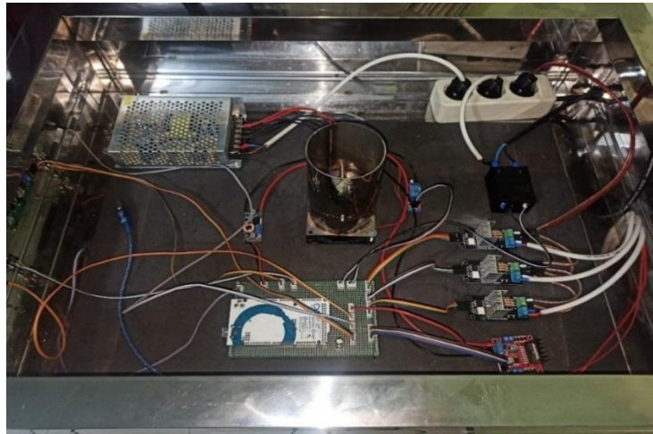
Figure 13. Electrical system
