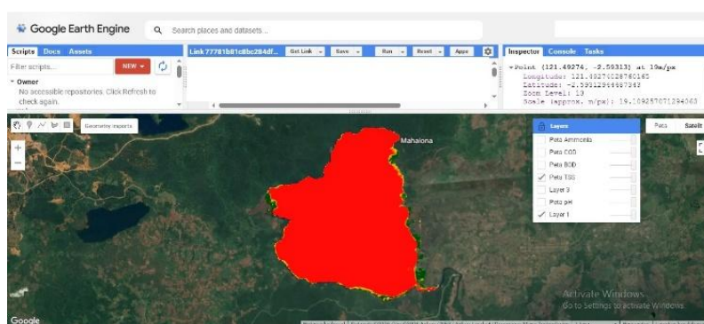
Figure 5 Visualization of Sentinel-2 Image Maps for the TSS Parameter in the Waters of Lake Mahalona for the Period (January 1, 2025 – November 1, 2025)
