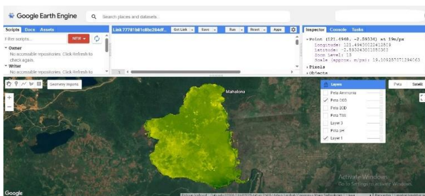
Figure 11. Visualization of Sentinel-2 Image Maps for COD Parameters in the Waters of Lake Mahalona for the Period (January 1, 2025 – November 1, 2025)
