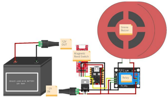
Figure 9. Wiring Components on a Motorcycle
