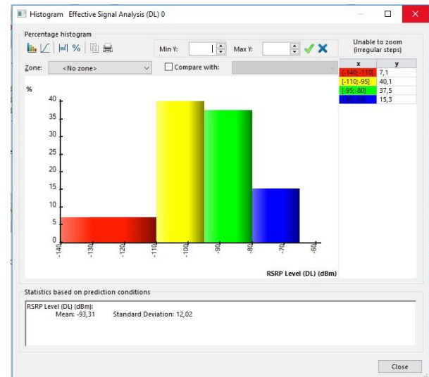
Gambar 5. Histogram Coverage Terhadap RSRP.
