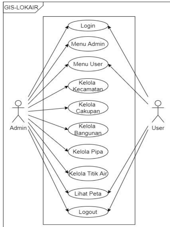
Gambar 1. Use case Diagram Sistem Usulan
