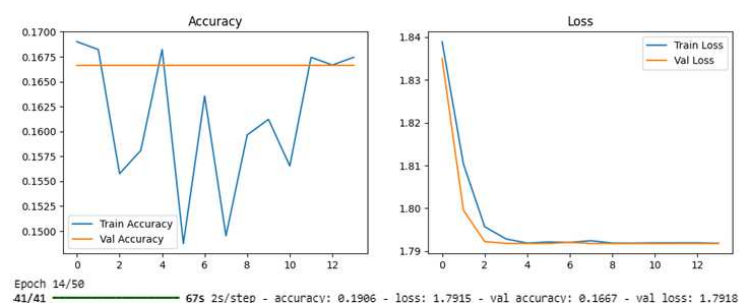
Gambar 8. Model EfficientNetB0
