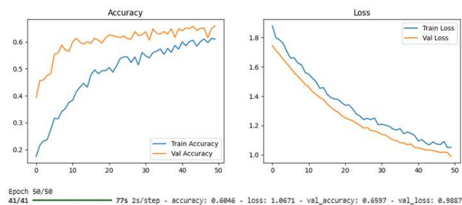
Gambar 7. Model VGG16
