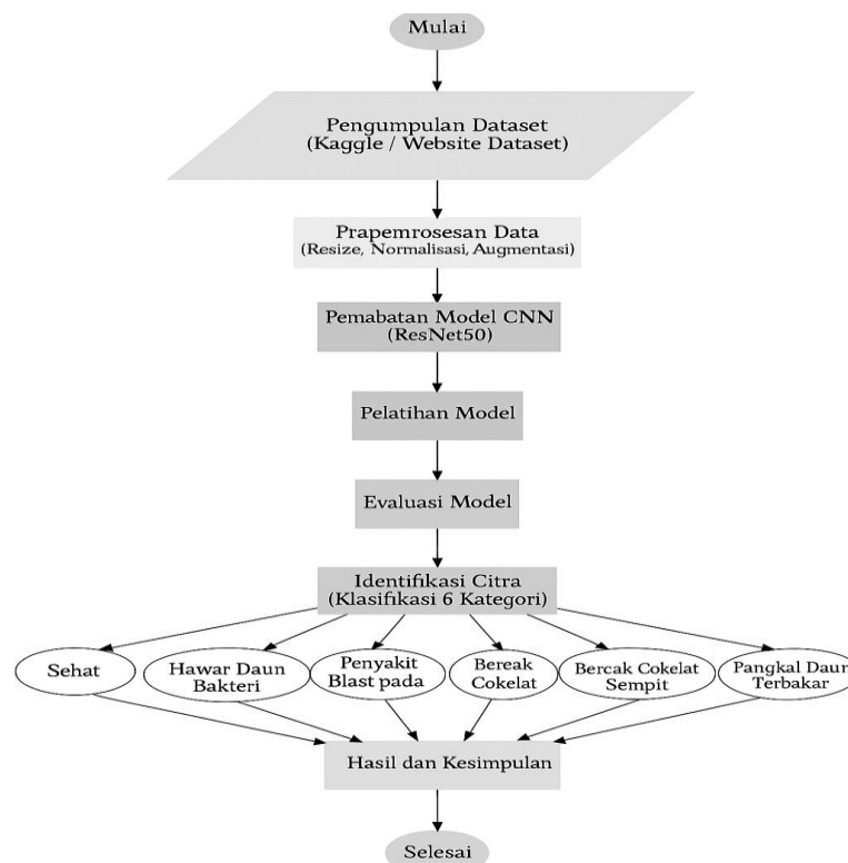
Gambar 1. Diagram Alur
