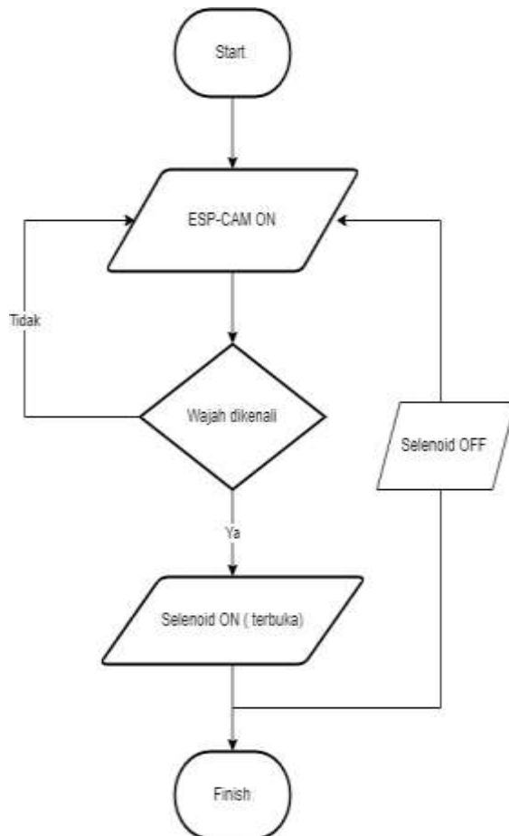
Gambar 5. Flowchart ESP-cam face recognition
