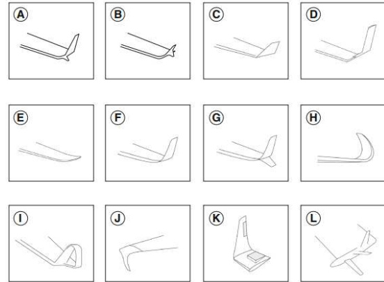
Gambar 2. a Whitcomb winglet. b Tip fence. c Canted winglet. d Vortex diffuser. e Raked winglet. f Blended winglet. g Blended split winglet. h Sharklet. i Spiroid winglet. j Downward canted winglet. k Active winglets. l Tip sails [11]
