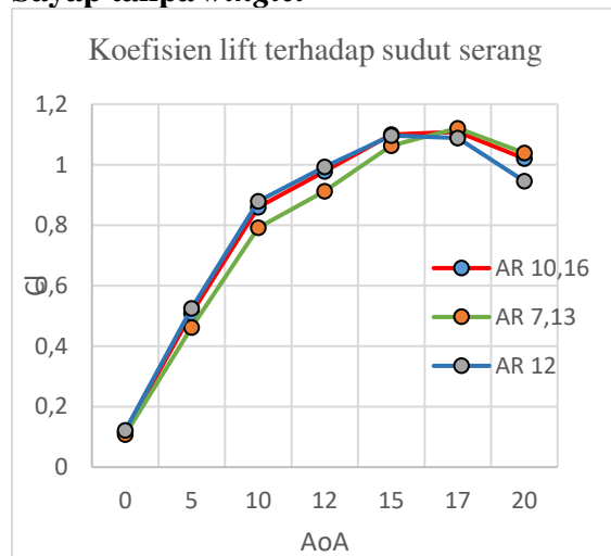
Gambar 5. Grafik C_l variasi aspect ratio
