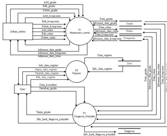
Gambar 3 DFD Level 0
