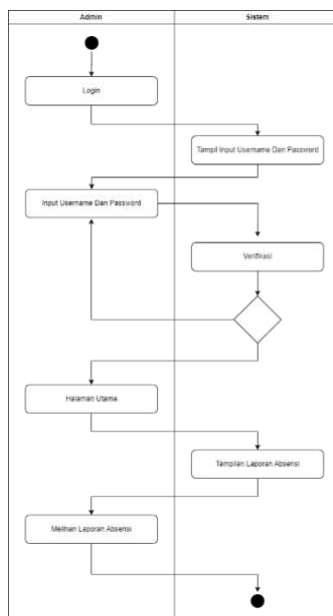
Gambar 3. Usecase Diagram
