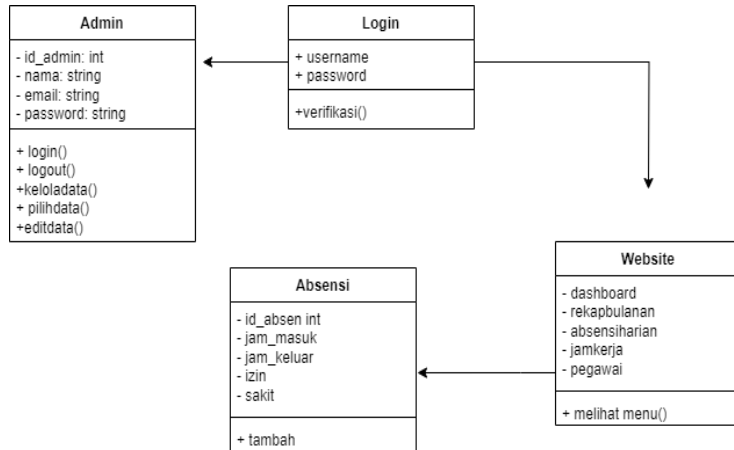
Gambar 4. Class Diagram
