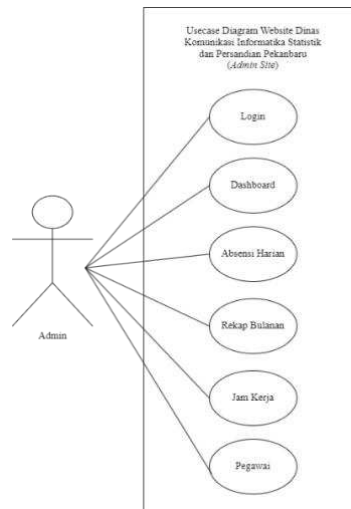
Gambar 2. Usecase Diagram
