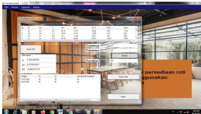
Gambar 5.8 Form Regresi
