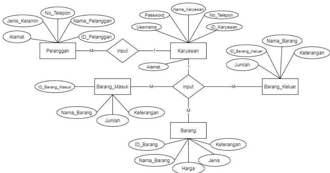
Gambar 3. ERD (Entity Relationship Diagram)
