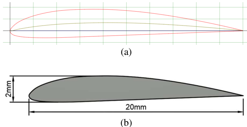
Gambar 1. (a) Acuan Airfoil Clark-Y (b) dimensi gambar potongan airfoil
