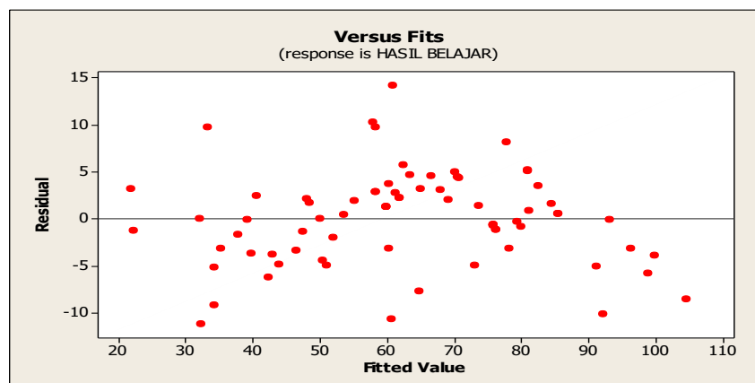
Gambar 1. Scatter Plot
