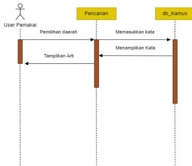
Gambar 5. Sequence Diagram
