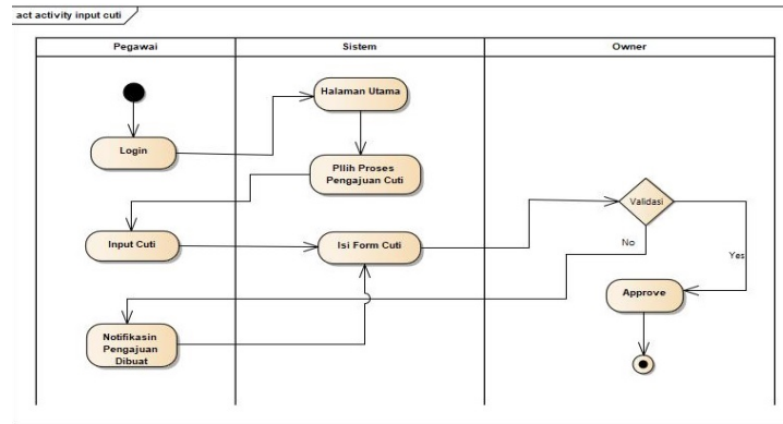
Gambar 9. Activity diagram Pegawai dan Owner
