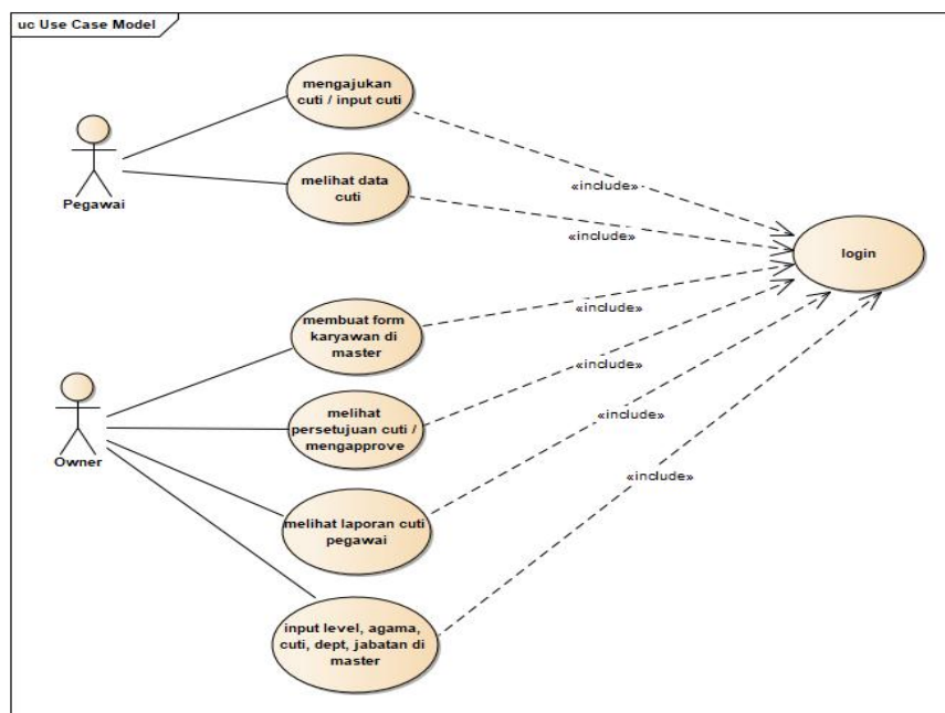
Gambar 8. Use Case Diagram Sistem
