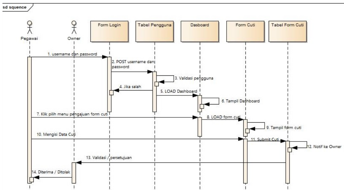
Gambar 12. Sequence diagram Pengajuan Cuti
