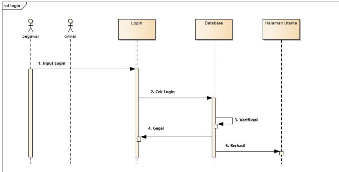
Gambar 11. Sequence diagram Login
