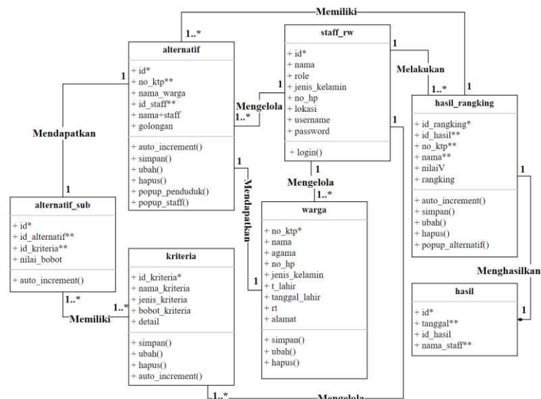
Gambar 2. Usecase Diagram
