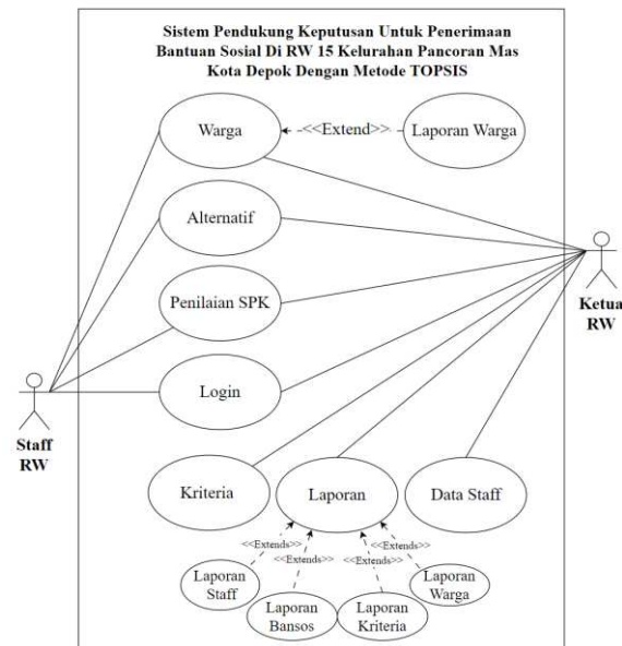
Gambar 1. Usecase Diagram
