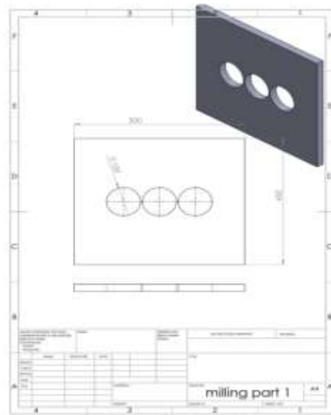
Gambar 4.6 Gambar Kerja Penelitian
