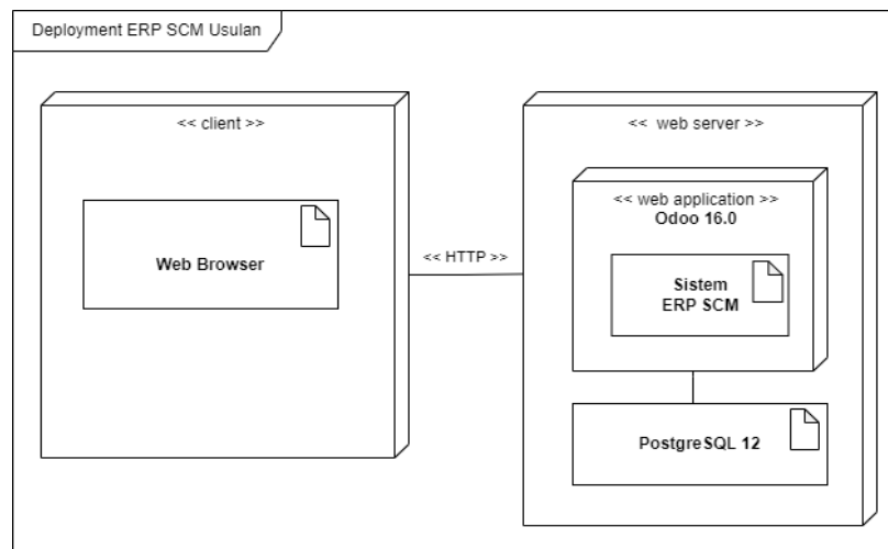
Gambar 6. Deployment Diagram
